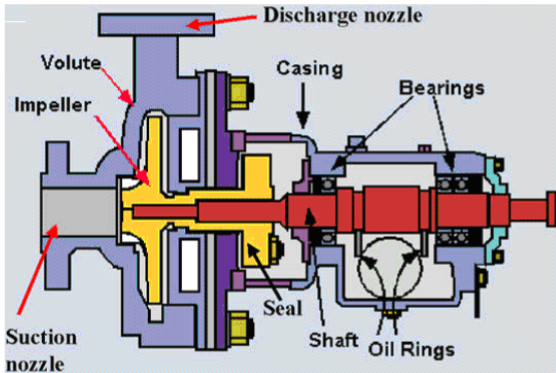
CENTRIFUGAL PUMP
